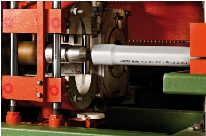
Details of the thermoforming process of the joint
